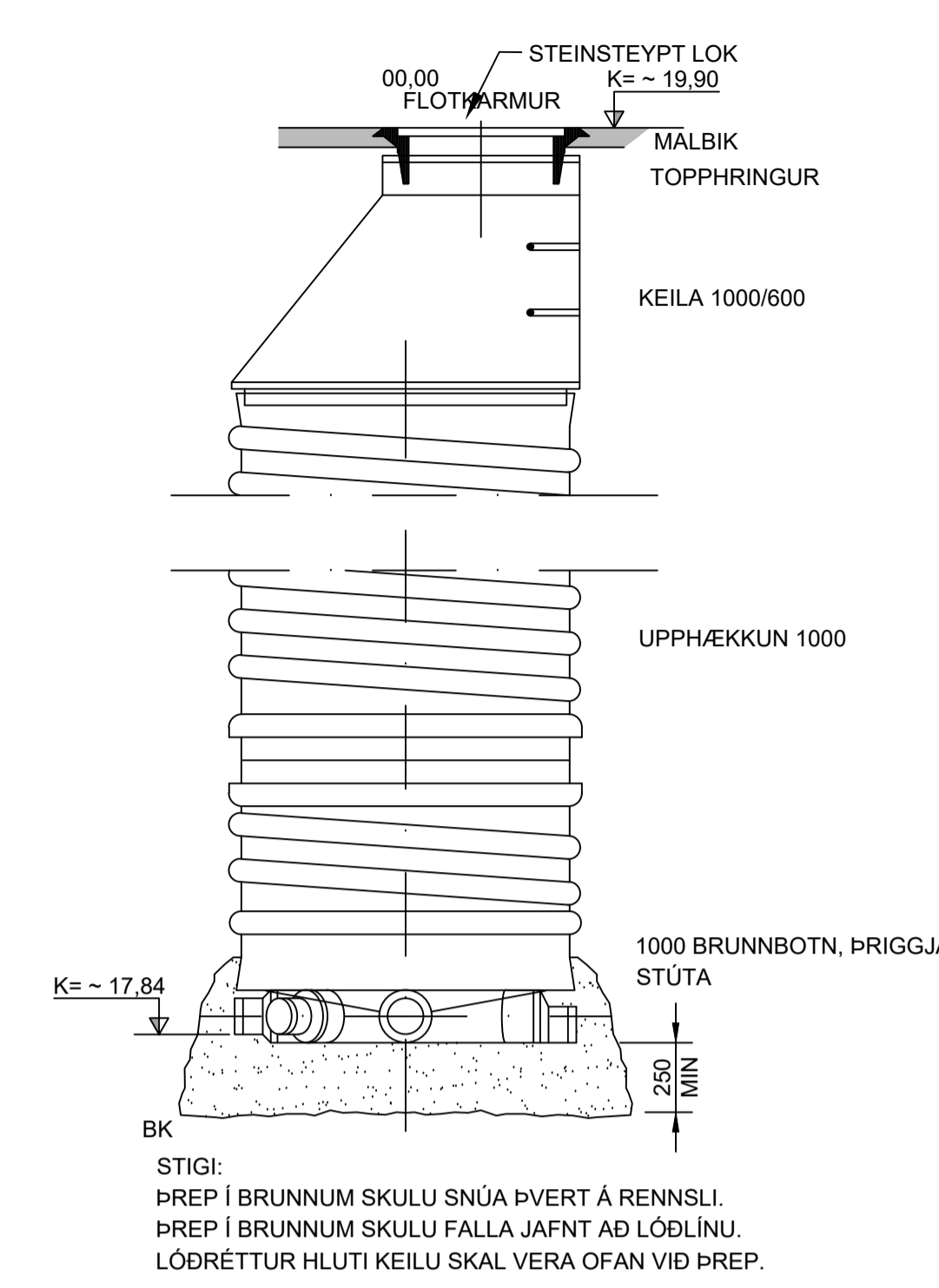
05 SNID - PASTBRUNNUR Ø1000 1011 1:20
