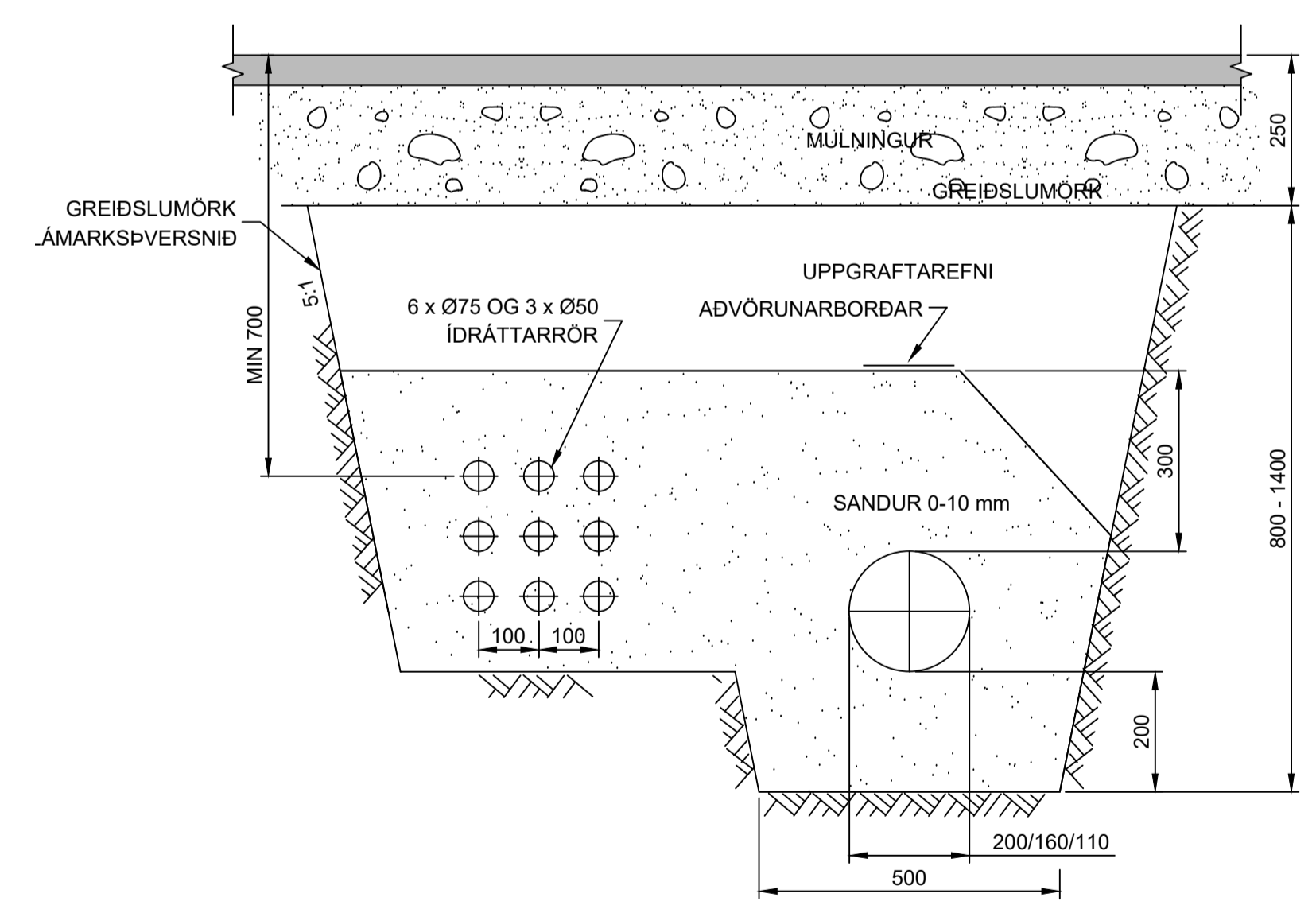
07 SNID 2301 1:10 1011 3S02
